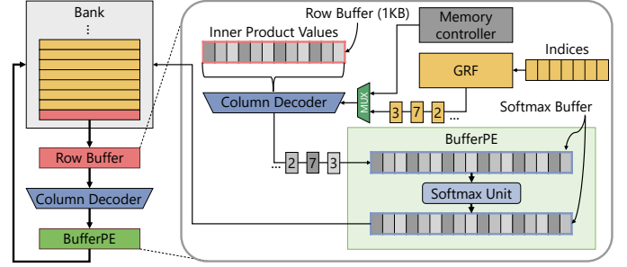
Fig. 8: Intra-row indirection for efficient random access.
